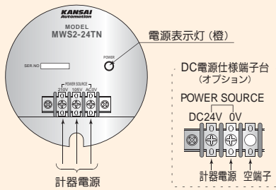
MWS2-24TN (送波器)
