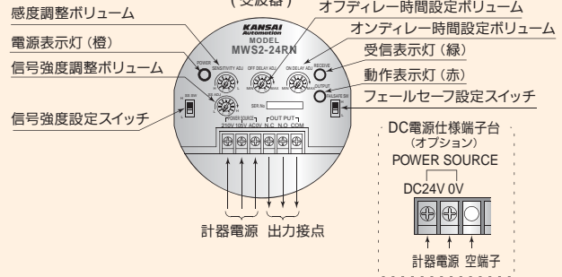
MWS2-24RN (受波器)
