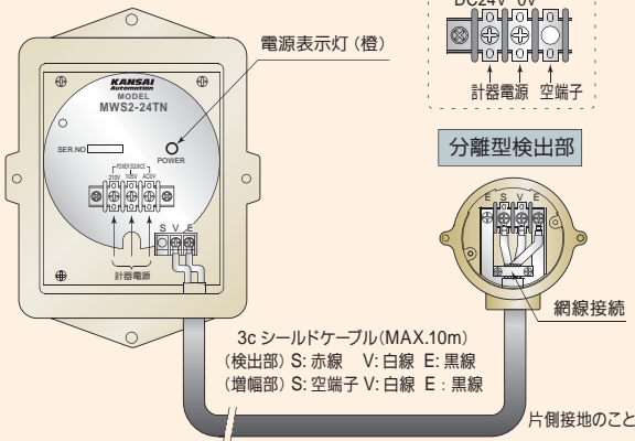
MWS2-24TN-R (送波器)
