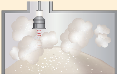
Malfunction by dust
