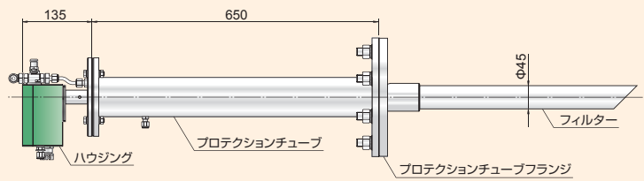
OXITEC 5000 (1400℃仕様)
