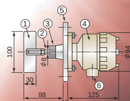
NL-8B (接粉部SUS)
